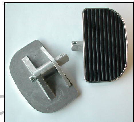
pedane comfort/floor boards
