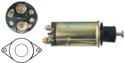
231251 Solenoid
