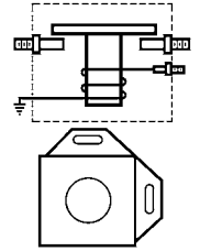
133855 Solenoid Replacing: SAZ-4201X, SAZ-4201R, SAZ-4201ENY, SAZ-4201ELY, SAZ-4201E, SAZ-4201CJ, SAZ-4201CA, SAZ-4201BR 12 V., 100 Amp., Intermittent load 800 Amp., Coil bolt M8 3.95-4.15 Coil resistance.
