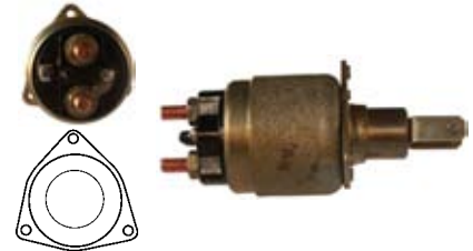
130367 Solenoid Replacing: 63600507 Servicing: 63222400, 63222430, 63222700, 63222701, 63222730, 63222731 12 V., Coil bolt M8 Cap: Cargo 131324.
