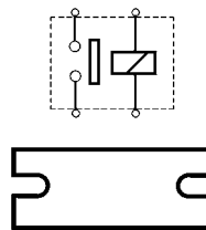
131373 Solenoid Replacing: 333009004 Servicing: 333009004 12 V., 150 Amp., Intermittent load 800 Amp., Seconds 5, Coil bolt M8 Silver contact. Insulated return.
