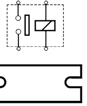
133695 Solenoid Replacing: CEY113, 099845 12 V., 100 Amp., Intermittent load 500 Amp., Seconds 5, Coil bolt M8
