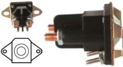
234072 Solenoid 12 V., 80 Amp., Coil bolt 5/16"-24 Insulated return.
