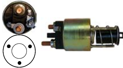
138444 Solenoid
