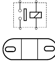
131253 Solenoid Replacing: 19024762 12 V., 60 Amp., Intermittent load 500 Amp., Seconds 5, Coil bolt M8
