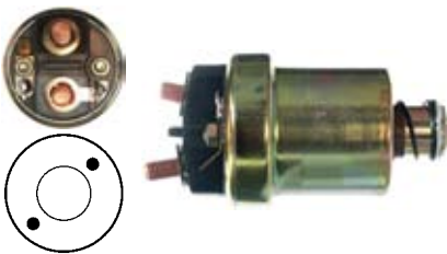
131010 Solenoid
