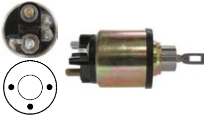
235107 Solenoid Replacing: 2339304035 Servicing: 0001106015 12 V., Coil bolt M8
