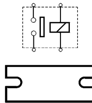
131371 Solenoid Replacing: 333006006 Servicing: 333006006 24 V., 80 Amp., Intermittent load 500 Amp., Seconds 5, Coil bolt M8 Silver contact. Insulated return.
