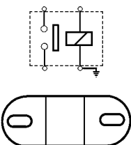
131080 Solenoid Replacing: 19024764 12 V., 50 Amp., Intermittent load 500 Amp., Seconds 5, Coil bolt M8
