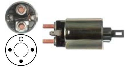
133052 Solenoid
