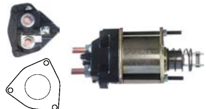
130377 Solenoid Replacing: 63902000, 63600400 Servicing: 63220700 12 V., Coil bolt M8 Cap: Cargo 131325.
