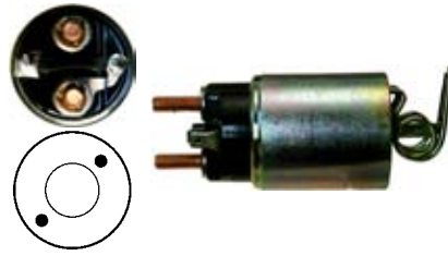
138811 Solenoid Servicing: S13-91 12 V., Coil bolt M8 Cap: Cargo 138812.
