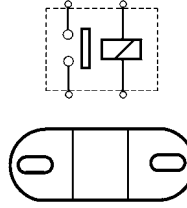
131254 Solenoid Replacing: 19024763 24 V., 50 Amp., Intermittent load 500 Amp., Seconds 5, Coil bolt M8
