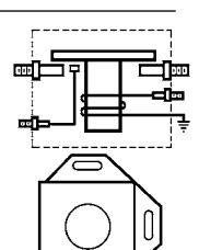
133856 Solenoid Replacing: SW1162 12 V., 100 Amp., Intermittent load 800 Amp., Coil bolt M8 3.95-4.15 Coil resistance.
