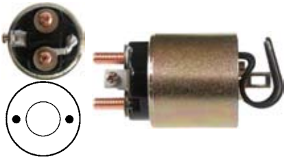
139832 Solenoid
