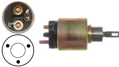
132265 Solenoid
