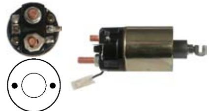
131084 Solenoid Replacing: 053400-3340, 053400-2557, 053400-2551, 053400-2160, 053400-1831, 053400-1830, 053400-1811 Servicing: 028000-1973, 028000-2000, 028000-3710, 028000-4042, 028000-4270, 028000-4330, 028000-4330, 028000-4331, 028000-4332 12 V., Coil bolt M8 Cap: Cargo 131374.
