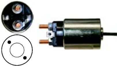
138739 Solenoid Replacing: 2130-47005, 2130-17010 Servicing: S13-115, S13-115A, S13-120A, S13-294, S13-94, S13-94A, S13-94A 12 V., Coil bolt M8
