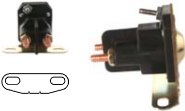
234073 Solenoid 12 V., 80 Amp., Coil bolt 1/4"-20 Insulated return.
