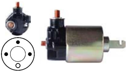
230018 Solenoid
