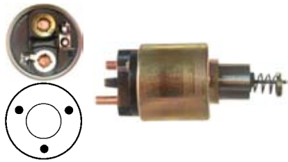
132261 Solenoid
