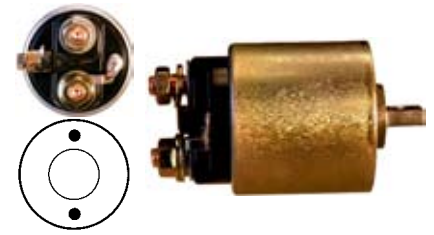
138957 Solenoid Replacing: 2114-27613 Servicing: S114-808, S114-869 12 V., Coil bolt M8 Cap: Cargo 139604.
