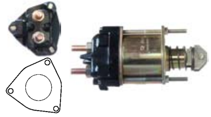
130361 Solenoid Replacing: 63600506, 63600504, 63600502 12 V., Coil bolt M8 Cap: Cargo 131326.
