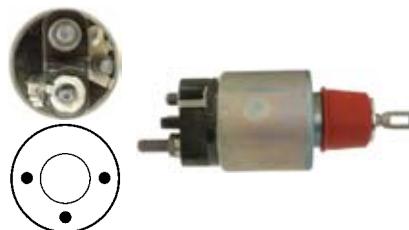
236516 Solenoid Replacing: 2339303422, 2339303387, 2339303355 Servicing: 0001123002, 0001123002, 0001123003, 0001123003, 0001125600, 0001125600, 0001125601, 0001125601 12 V., Coil bolt M8
