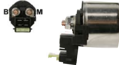
235593 Solenoid 12 V. 20 Amp. Fuses.
