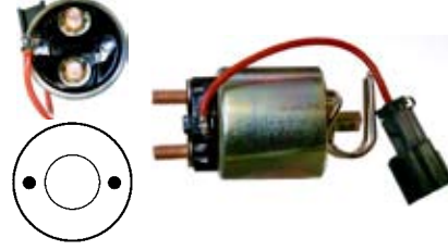
138823 Solenoid Replacing: 2114-97605 Servicing: S114-527, S114-527A, S114-527B 12 V., Coil bolt M8 Cap: Cargo 138819.
