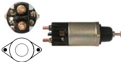
234292 Solenoid
