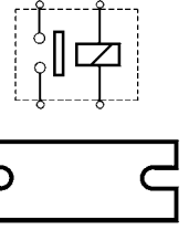
133697 Solenoid Replacing: CEZ113, 098932 24 V., 100 Amp., Intermittent load 500 Amp., Seconds 5, Coil bolt M8
