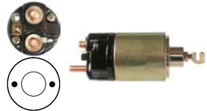
130814 Solenoid Replacing: 053400-3810, 053400-3720, 053400-3710, 053400-3410, 053400-3350, 053400-3330, 053400-2880 Servicing: 028000-1850, 028000-1975, 028000-1975, 028000-1975, 028000-1976, 028000-1976, 028000-1976, 028000-2001, 028000-2150 12 V., Coil bolt M8 Cap: Cargo 134627.
