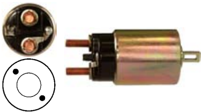
138809 Solenoid Replacing: 2130-37005 Servicing: S13-104 12 V., Coil bolt M8 Cap: Cargo 138810.
