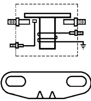
130493 Solenoid Replacing: 3225629, 2098360 12 V., Intermittent load 150 Amp., Coil bolt 5/16" UNF Insulated return. Flat Bracket.
