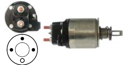
130373 Solenoid Replacing: 063602290010 Servicing: 063224600010, 063224602010, 063224691010 12 V., Coil bolt M8 Cap: Cargo 131327.
