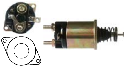
234544 Solenoid Replacing: 1350-114-02X9 Servicing: 0350-502-0047, 0351-502-0042 24 V., Coil bolt M10
