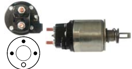
130373 Solenoid Replacing: 63602290, 63602200 Servicing: 63224600, 63224602, 63224691 12 V., Coil bolt M8 Cap: Cargo 131327.
