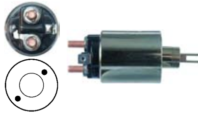
133047 Solenoid
