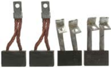
140873 Brush Set
