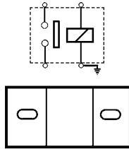
130492 Solenoid Replacing: 19024765 24 V., 50 Amp., Intermittent load 500 Amp., Seconds 5, Coil bolt M8
